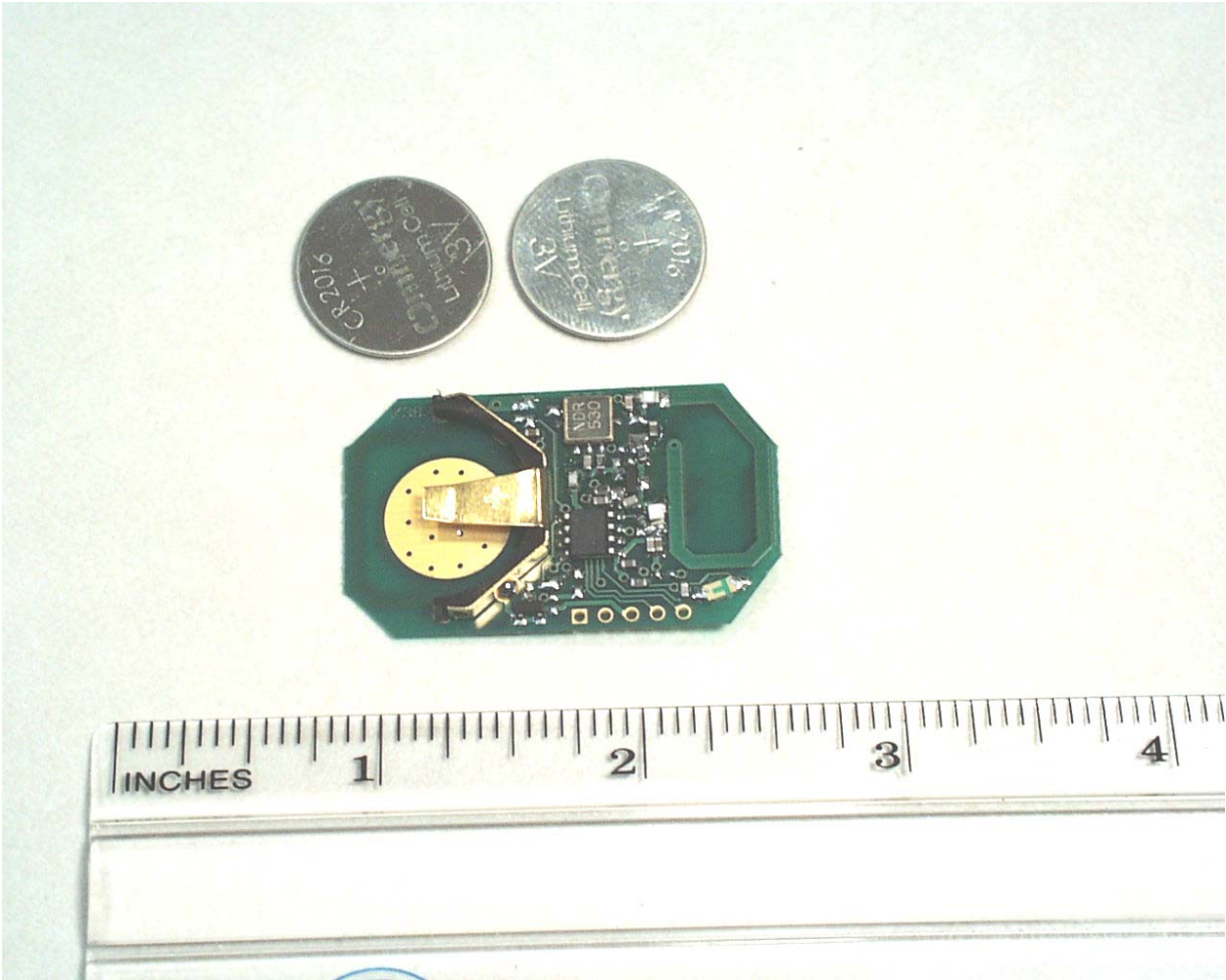
View of the Component Side of the PCB
