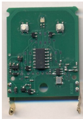
Annex 1A: S8TL318E2 – Electronic card front internal view
