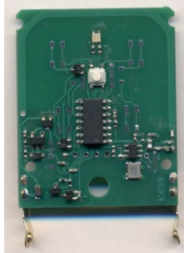
Annex 1A: S8TL318E1 – Electronic card front internal view
