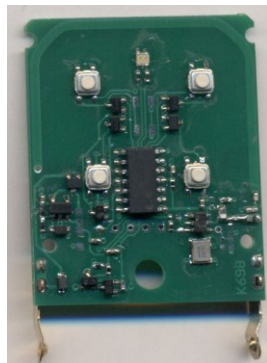
Annex 1A: S8TL318E4 – Electronic card front internal view
