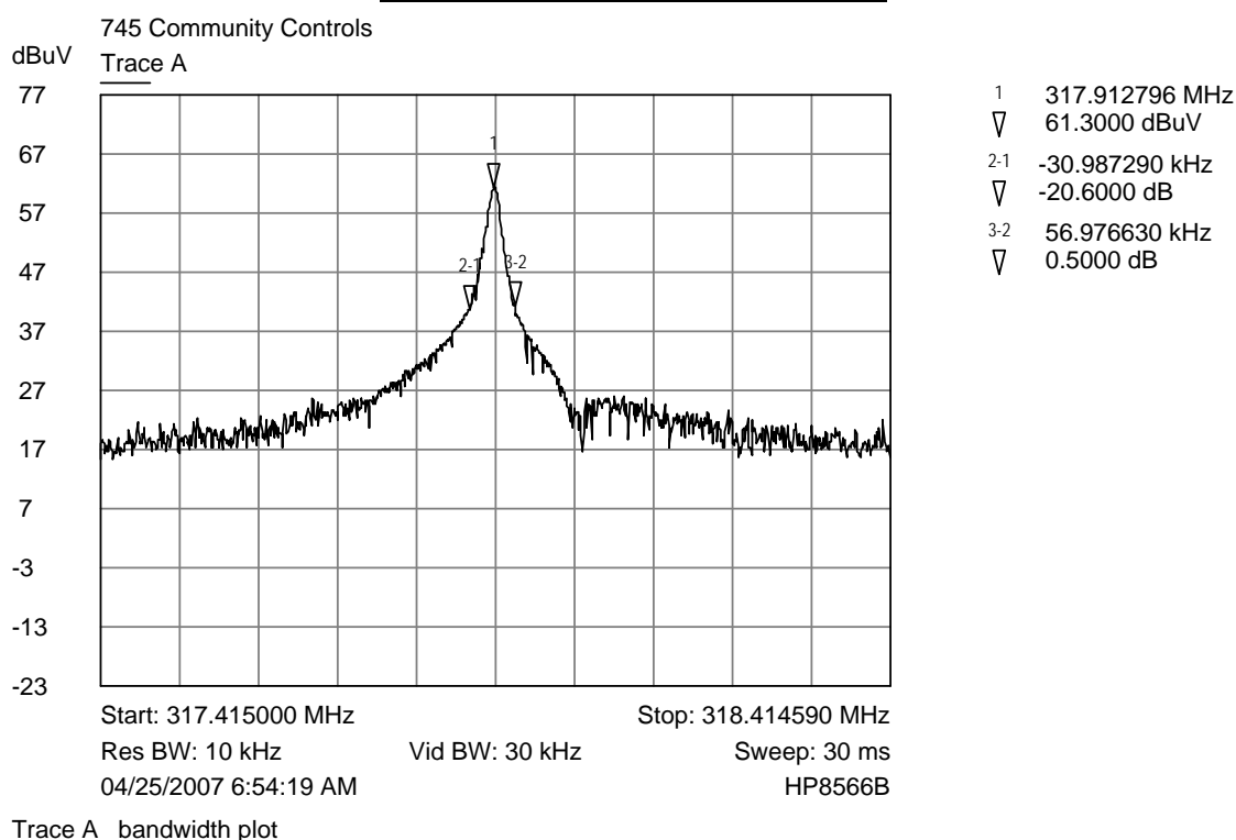
318LIPW1V Bandwidth Plot
