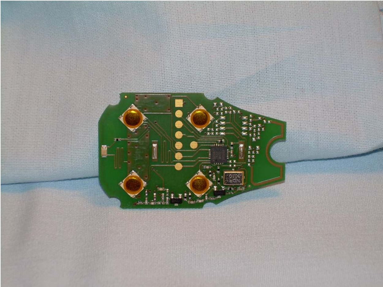
Button Side of the PCB
