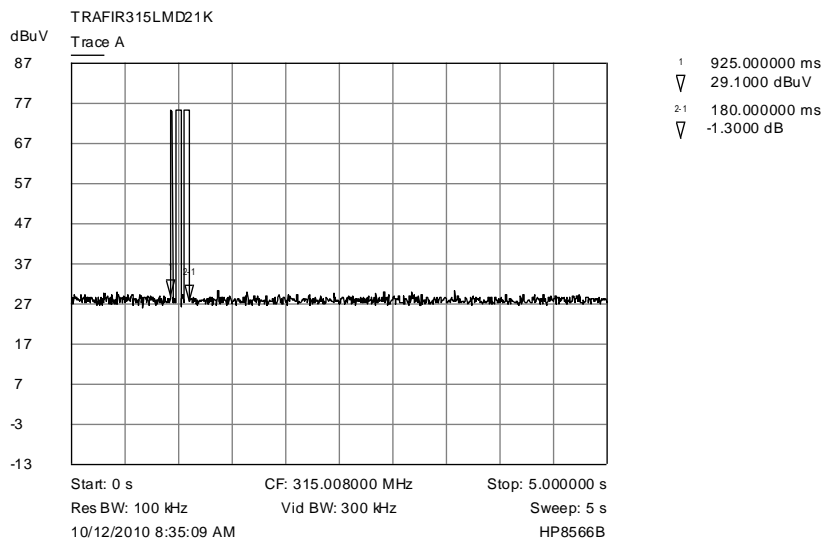
TRAFIR315LMD21K Trace A button pressed to transmit and then released
