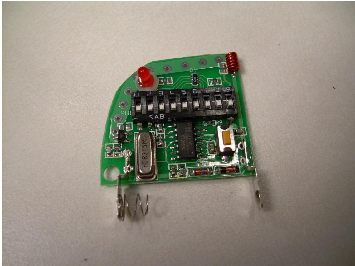
Photograph 7 – Component Side of PCB
