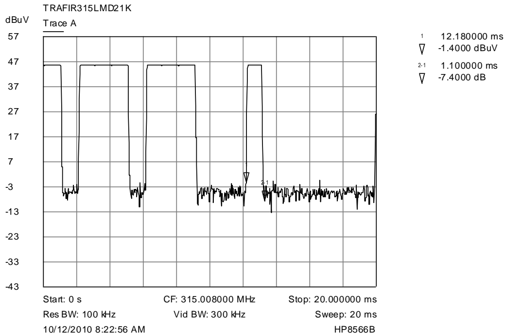
TRAFIR315LMD21K Trace A stop pulse timing
