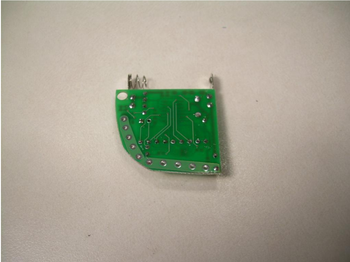
Photograph 8 – Trace Side of PCB
