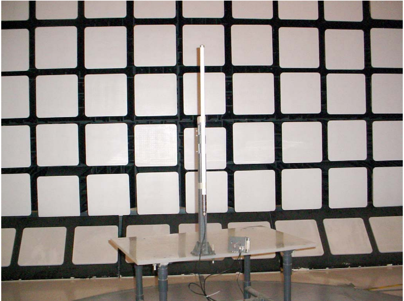
Radiated Emissions at 3 m EUT with 12 dBi Omni-directional Antenna (Orthogonal Position 3)
