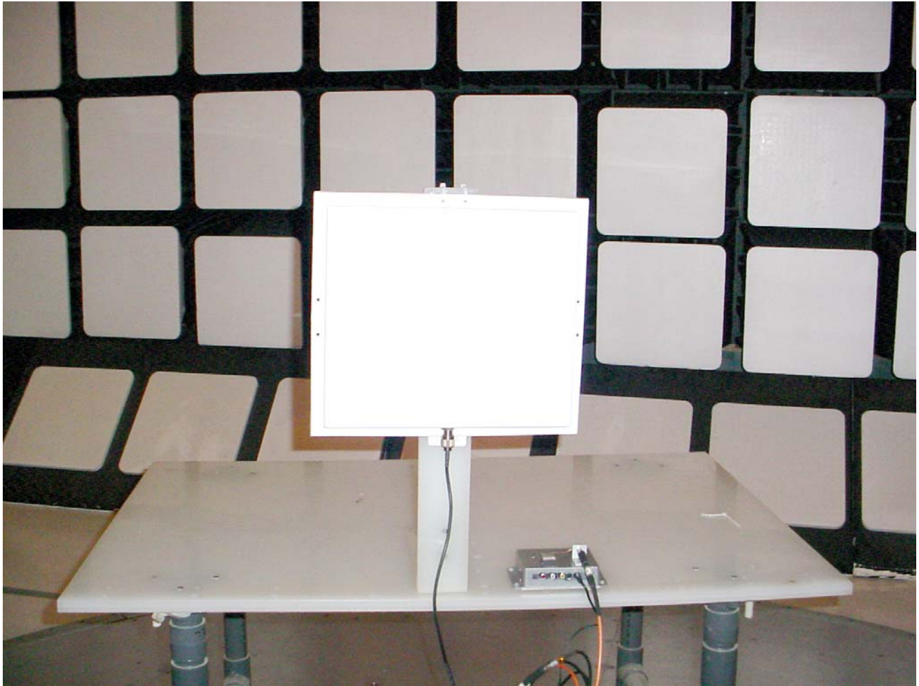
Radiated Emissions at 3 m EUT with 20.5 dBi Panel Antenna
