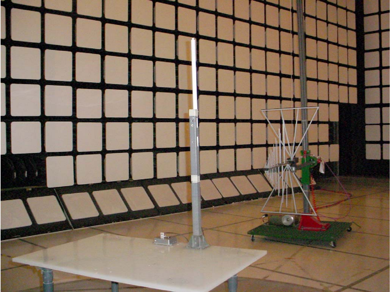
Radiated Emissions at 3 m EUT with 12 dBi Omni-directional Antenna (Orthogonal Position 1)
