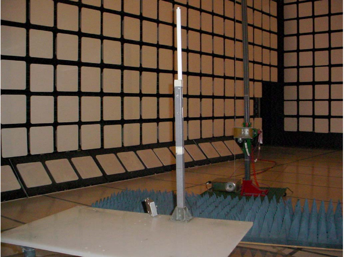
Radiated Emissions at 3 m EUT with 12 dBi Omni-directional Antenna
