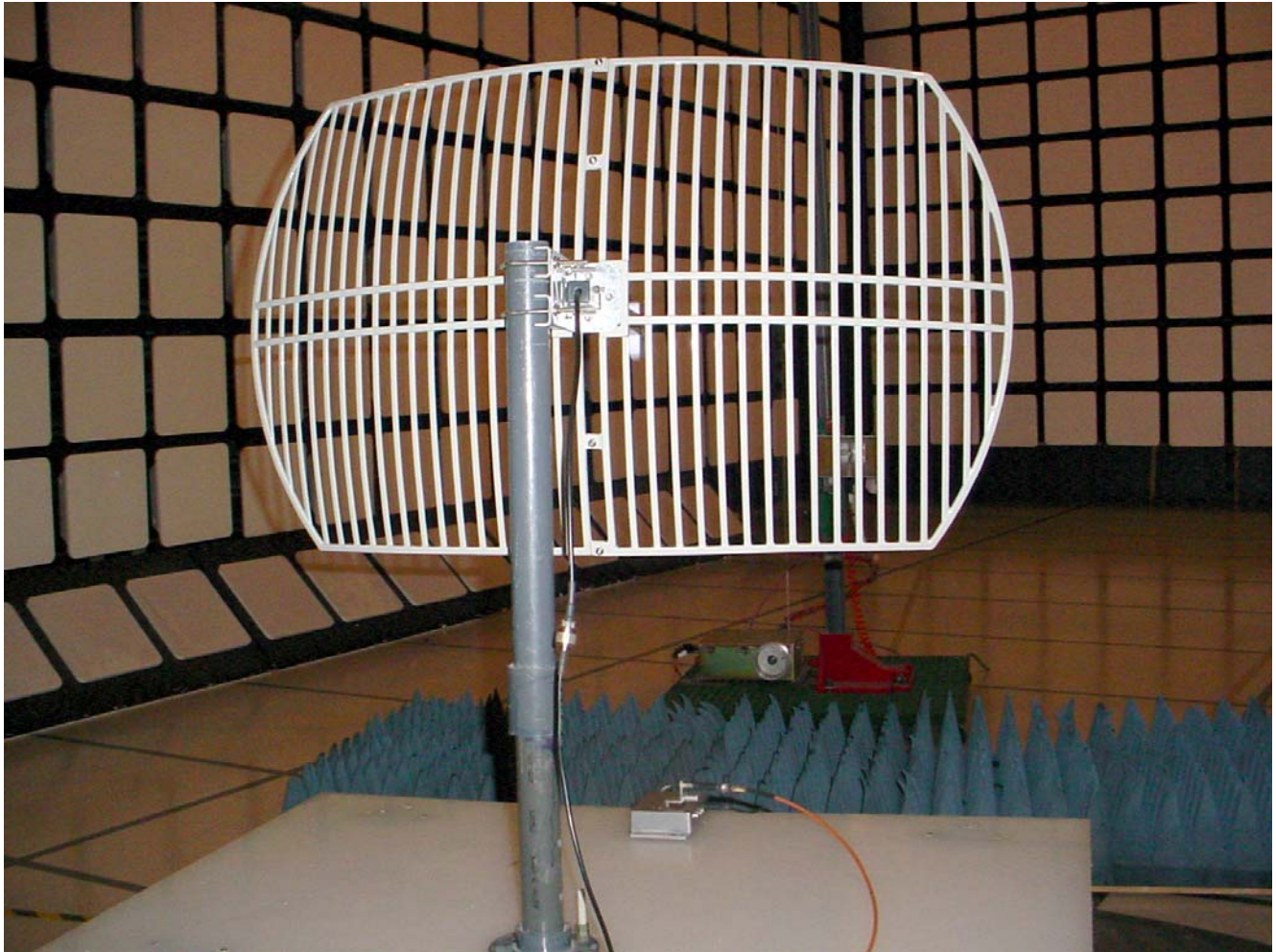
Radiated Emissions at 3 m EUT with 24 dBi Parabolic Antenna
