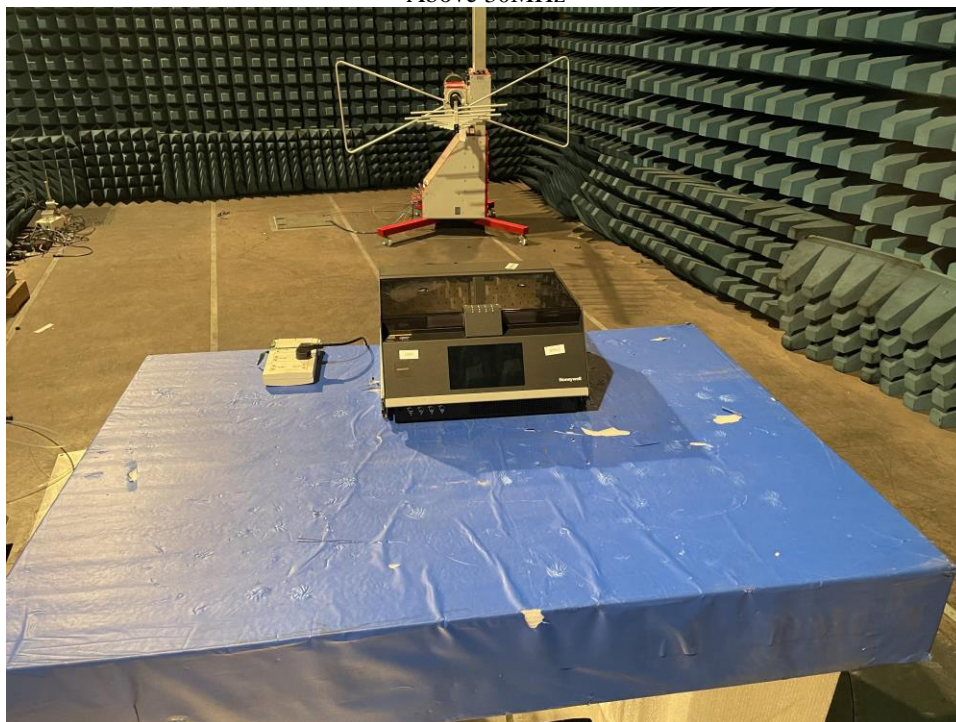
Above 30MHz
