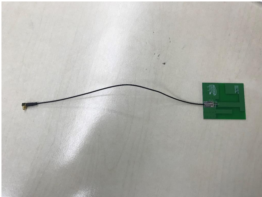
PCB antenna
