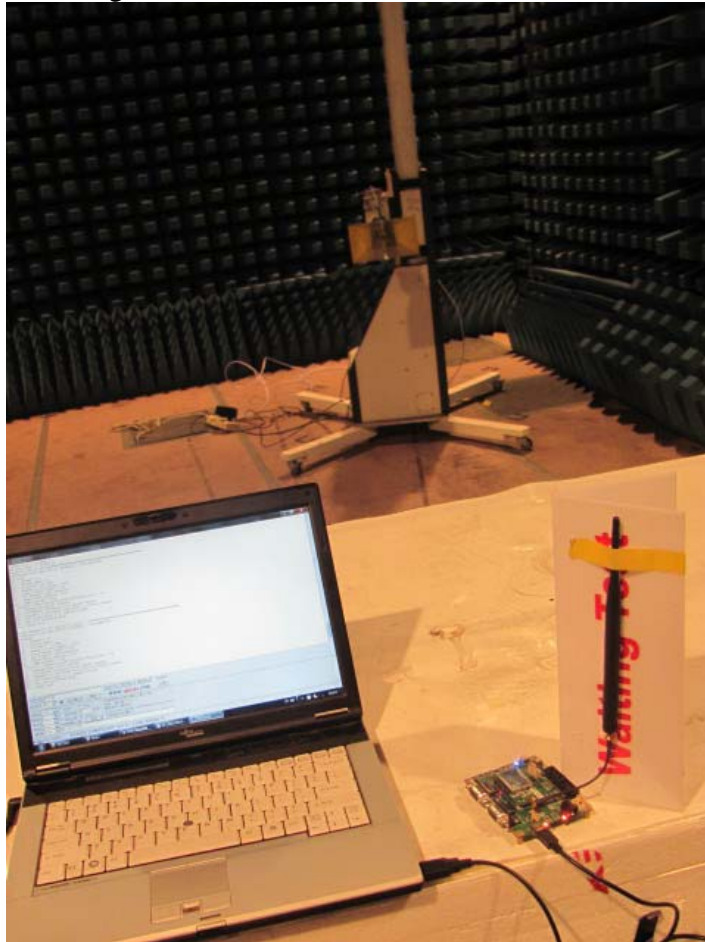
Higher than 1GHz, Omnidirectional Antenna
