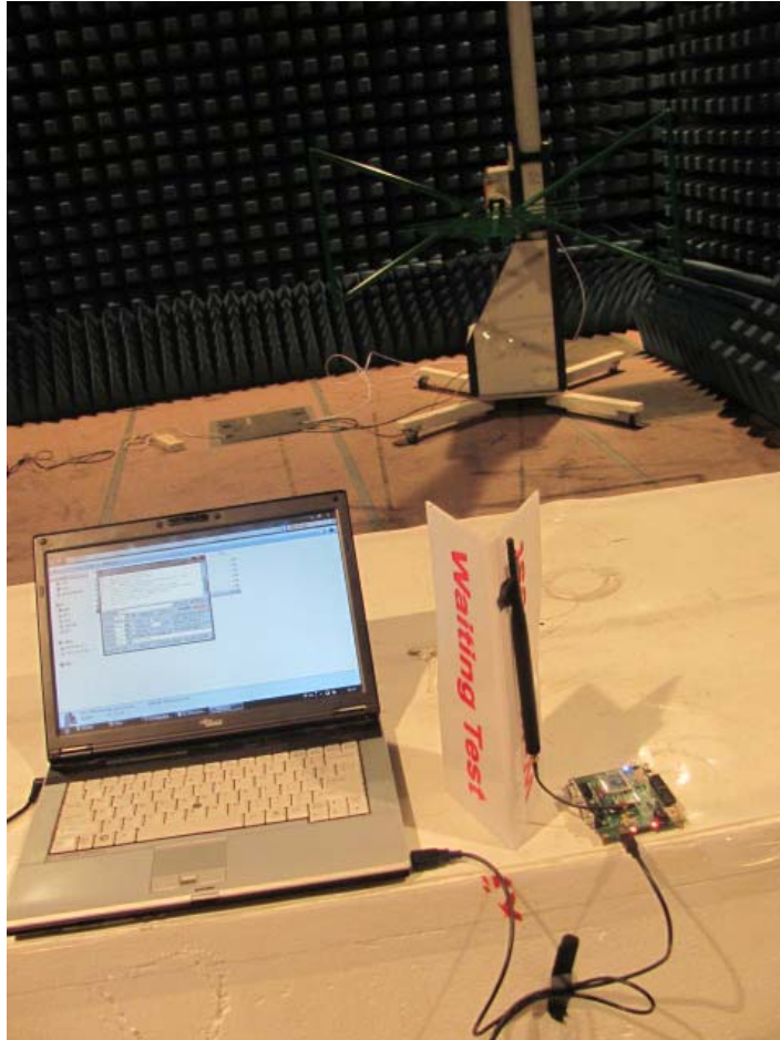
30MHz-1000MHz, Omnidirectional Antenna
