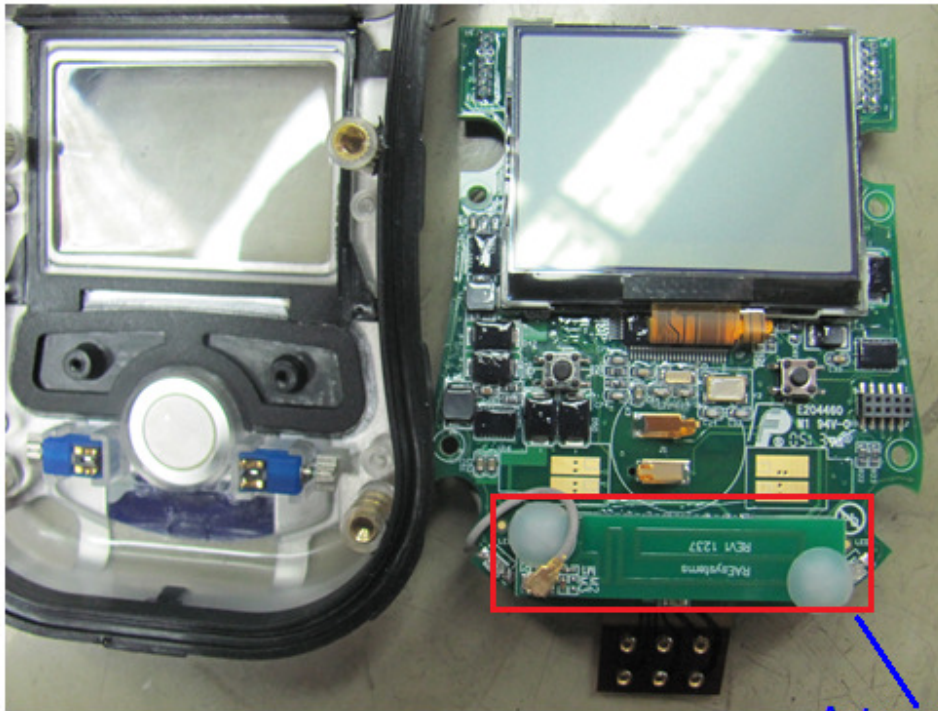
Antenna location
