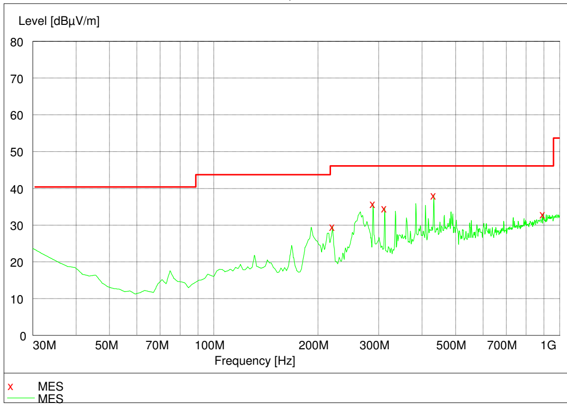
30MHz~1GHz, Horizontal
