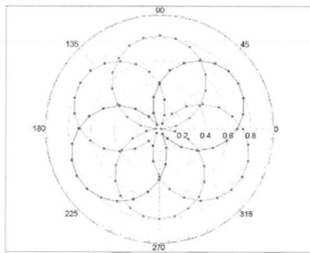
f=600 MHz,TEM
