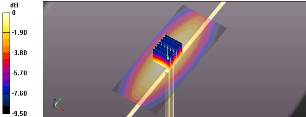
SAR MEASUREMENT PLOT 10
