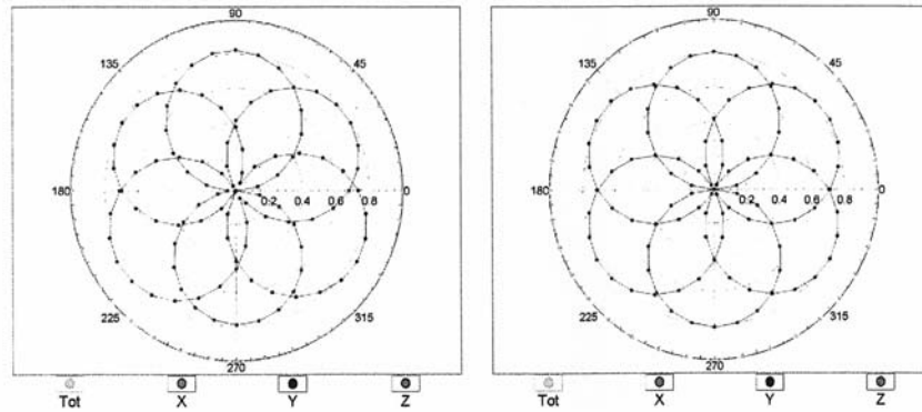
f=600 MHz,TEM
