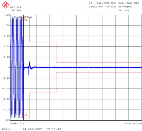
155.7525_Turn On
