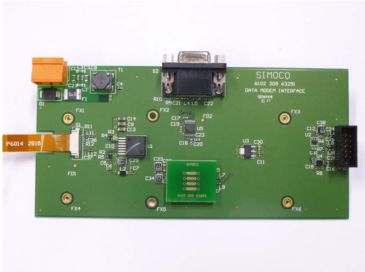
Serial Interface – Top
