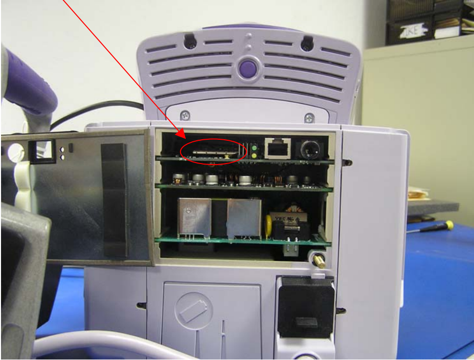
Closeup of EUT inside host
