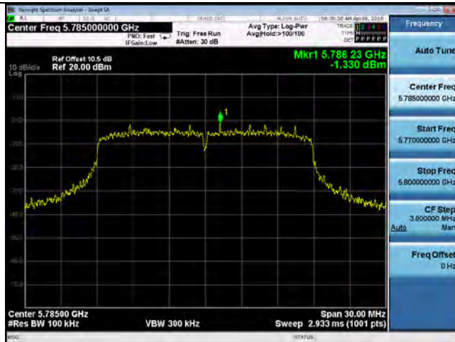
PSD-802.11n-20M 5785MHz Chain 1
