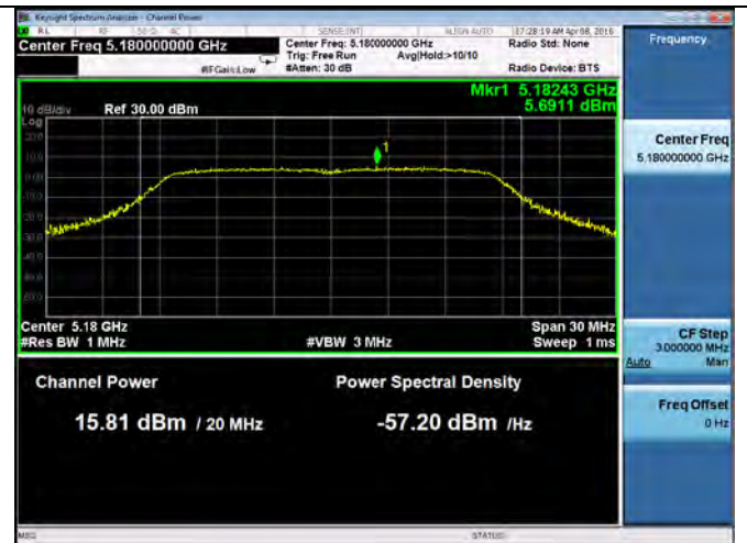
PSD-802.11n-20M-5180M (Chain 2)
