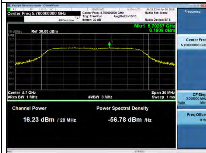
PSD-802.11n-20M-5700M (Chain 1)
