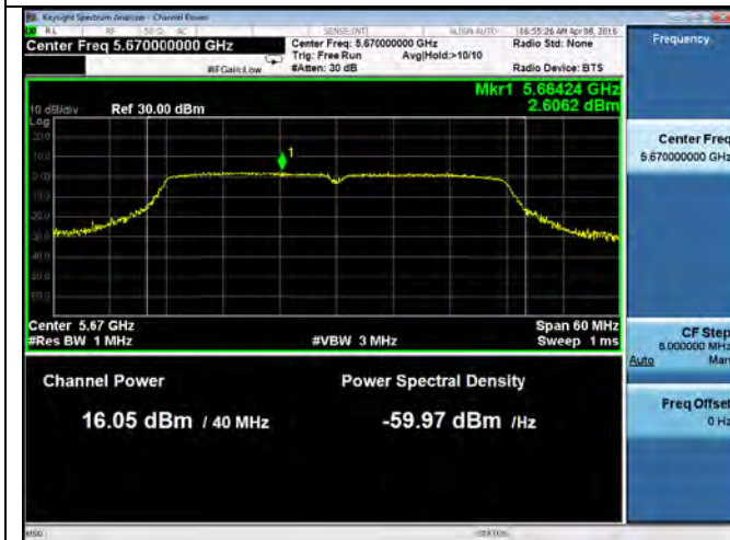
PSD-802.11n-40M-5670M (Chain 1)
