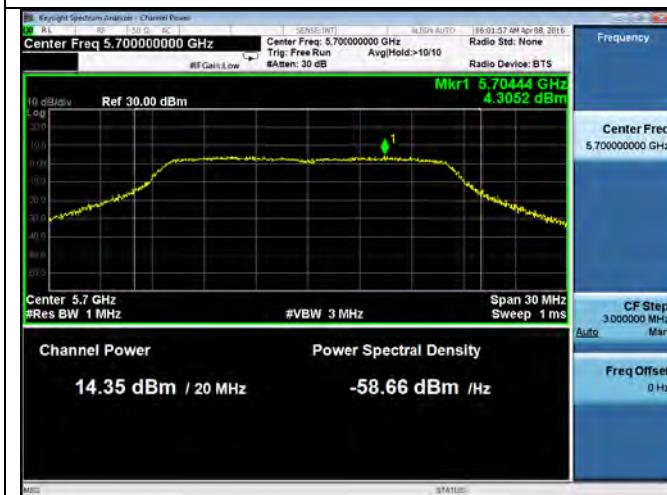
PSD-802.11a-5700M (Chain 1)
