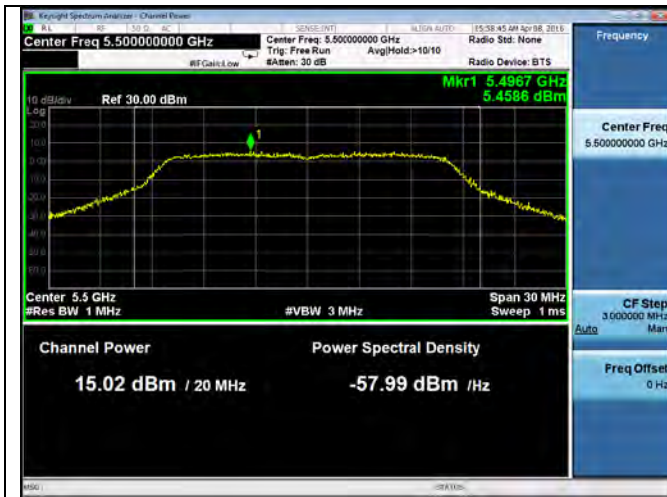
PSD-802.11a-5500M (Chain 1)
