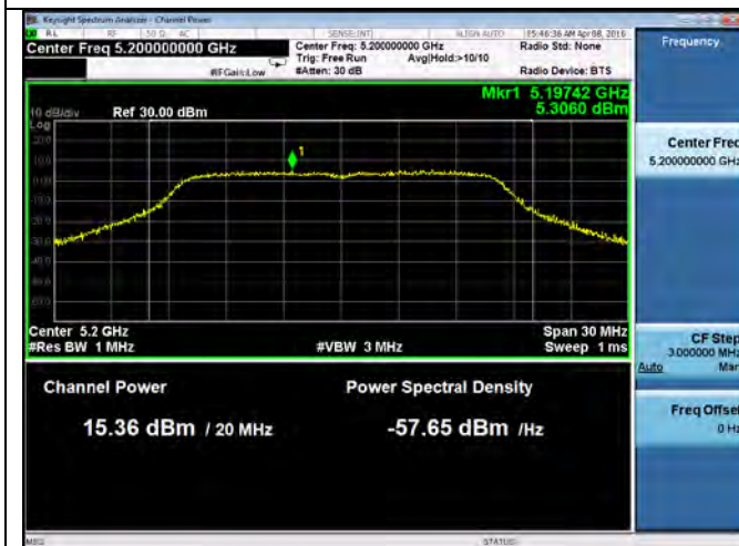
PSD-802.11a-5200M (Chain 1)
