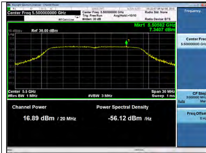
PSD-802.11n-20M-5500M (Chain 1)
