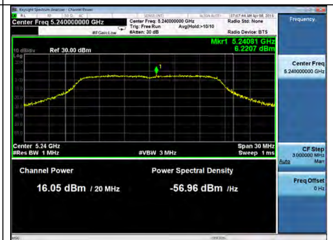
PSD-802.11a-5240M (Chain 2)
