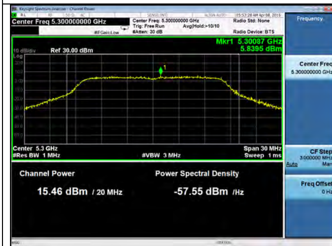
PSD-802.11a-5300M (Chain 1)
