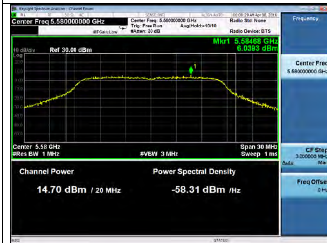
PSD-802.11a-5580M (Chain 1)
