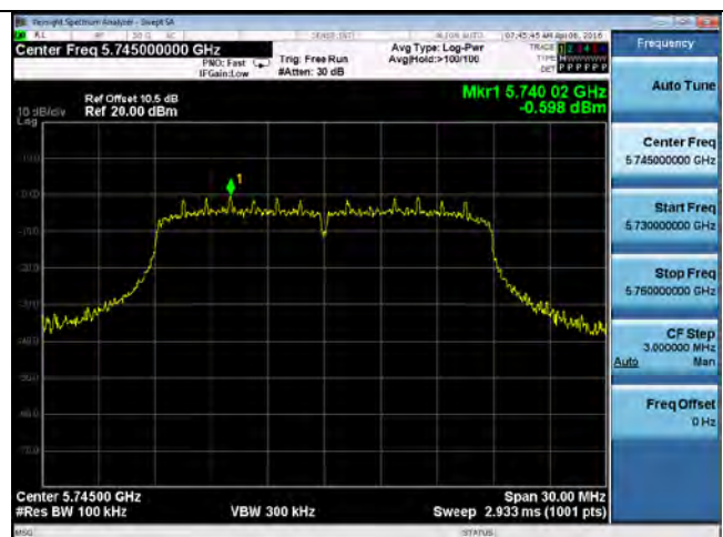
PSD-802.11n-20M 5745MHz Chain 2
