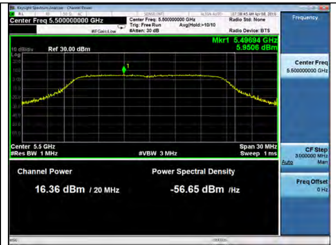
PSD-802.11n-20M-5500M (Chain 2)
