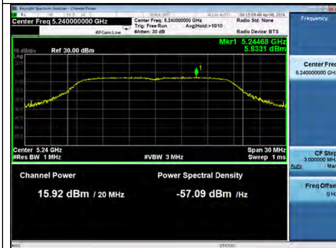
PSD-802.11n-20M-5240M (Chain 1)
