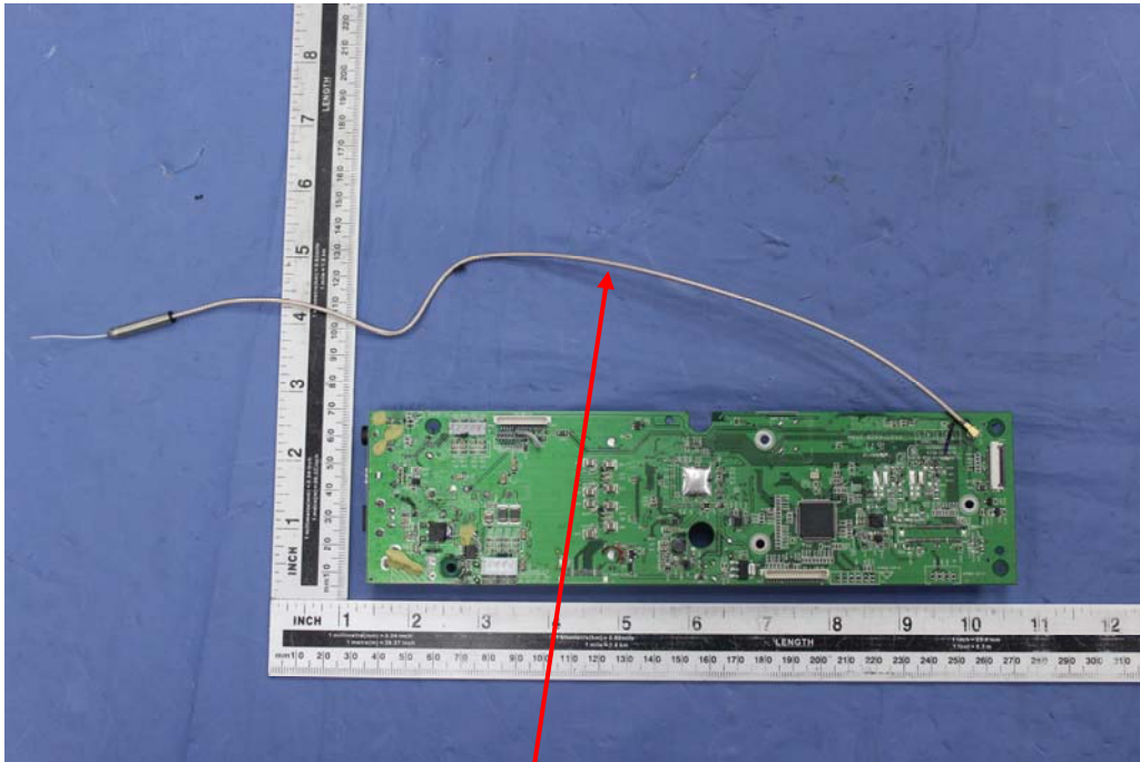
BT Antenna
