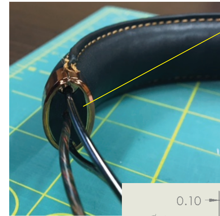
Die cuts are made to go around the spring wire and the headphone cable.
