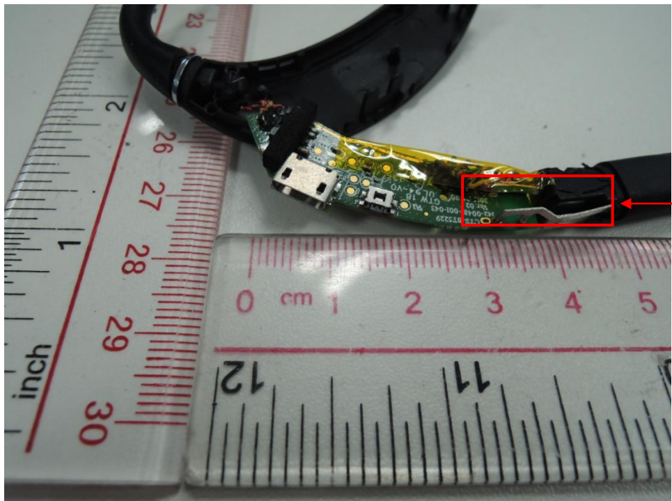
BT Antenna
