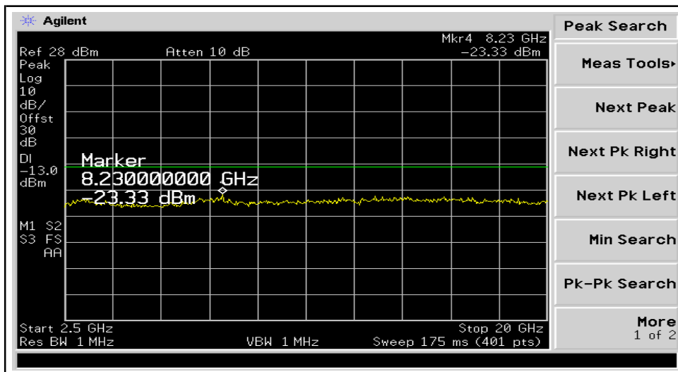
PLOTS OF EMISSION (CDMA): Out of Band(Ch1175)
