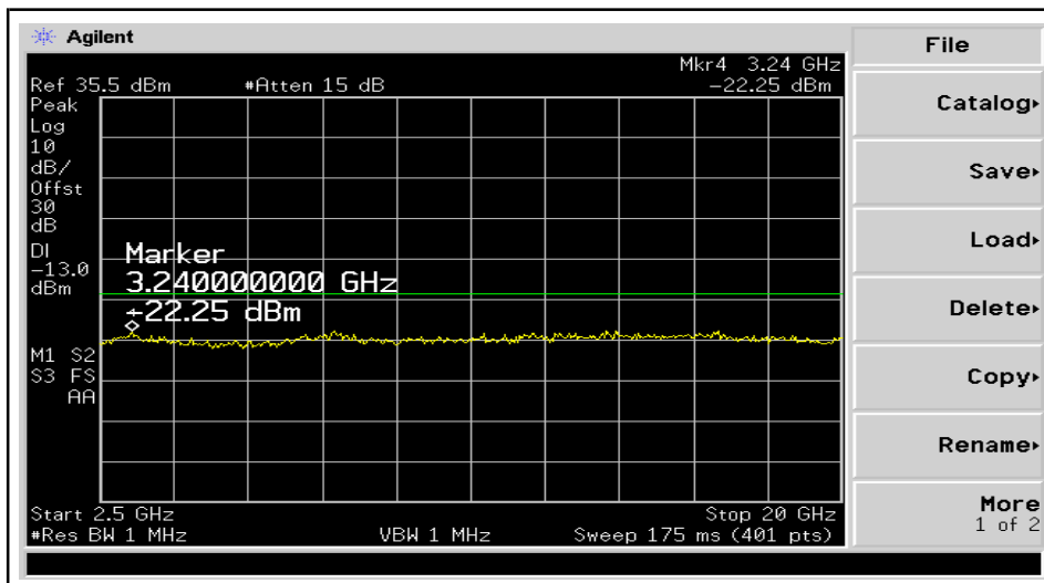
PLOTS OF EMISSION (GSM): Out of Band(Ch1175)
