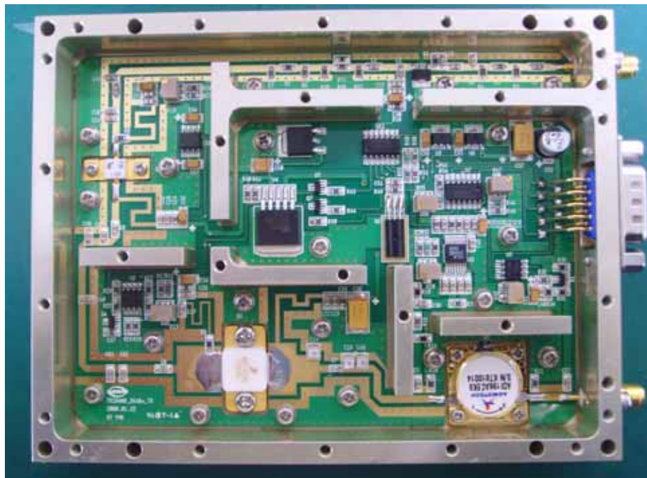
<RSN-TRI-25/24-DC DL HPA Top View>
