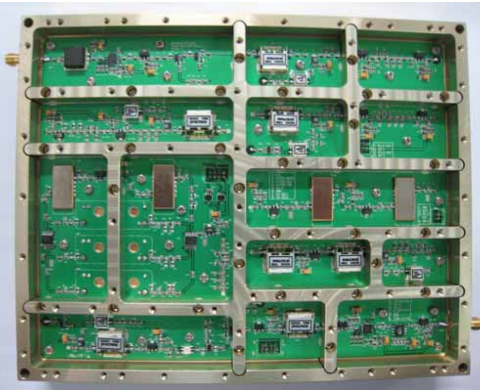
<RSN-TRI-25/24-DC DL Top View>
