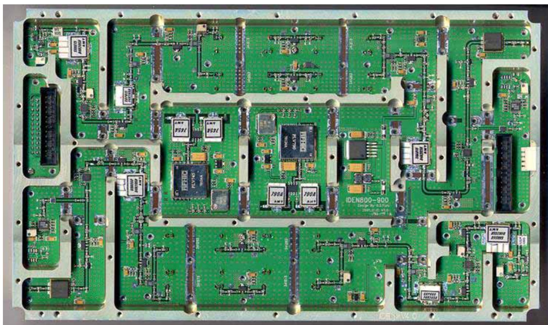
<RSN-iDEN-30 UDC Top view>
