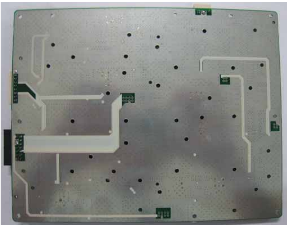
<CDMA DL PCB Bottom View>
