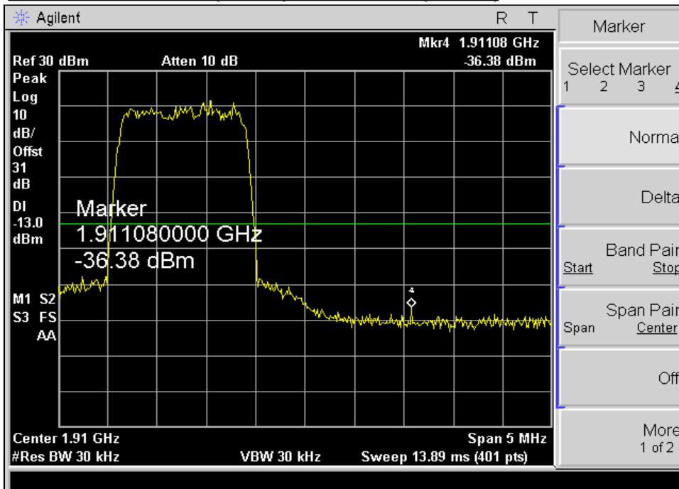
PLOTS OF EMISSION (CDMA): BAND EDGE(Ch1175)
