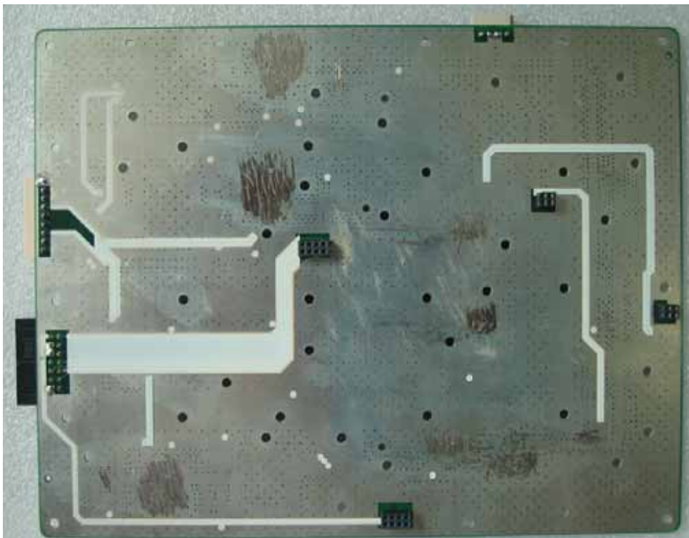
< CDMA 30 UL PCB Bottom View >
