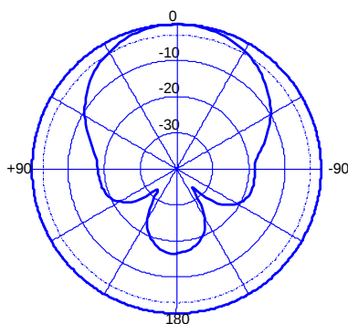
Horizontal Pattern
