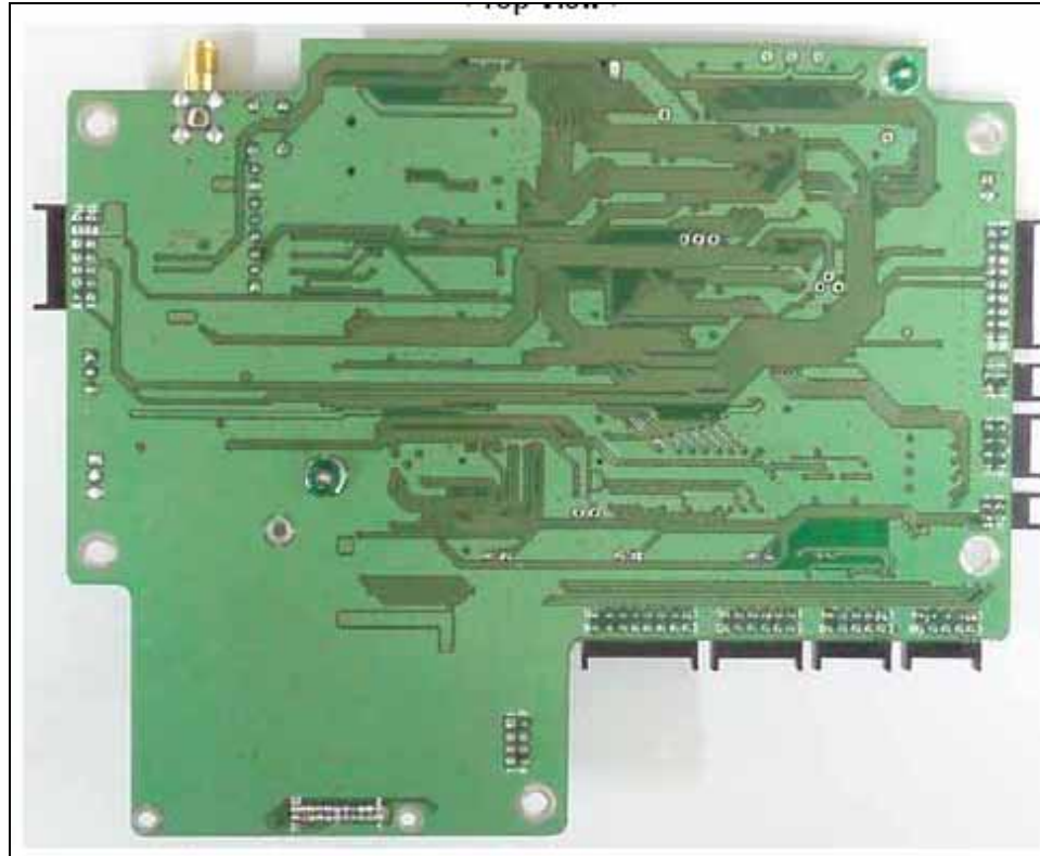
Bottom view of MCU Board
