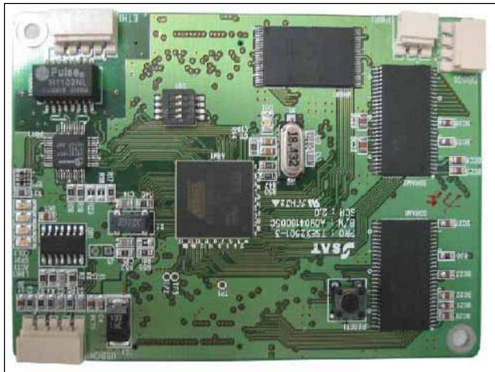
Top view of CPU Board
