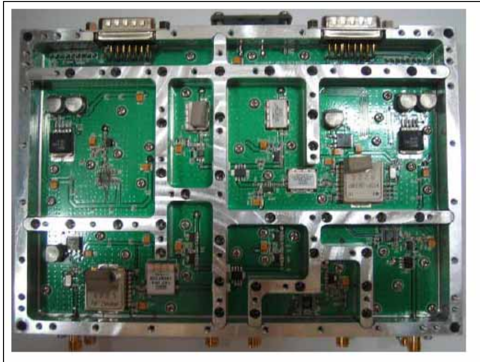
Top view of Digital Filter
