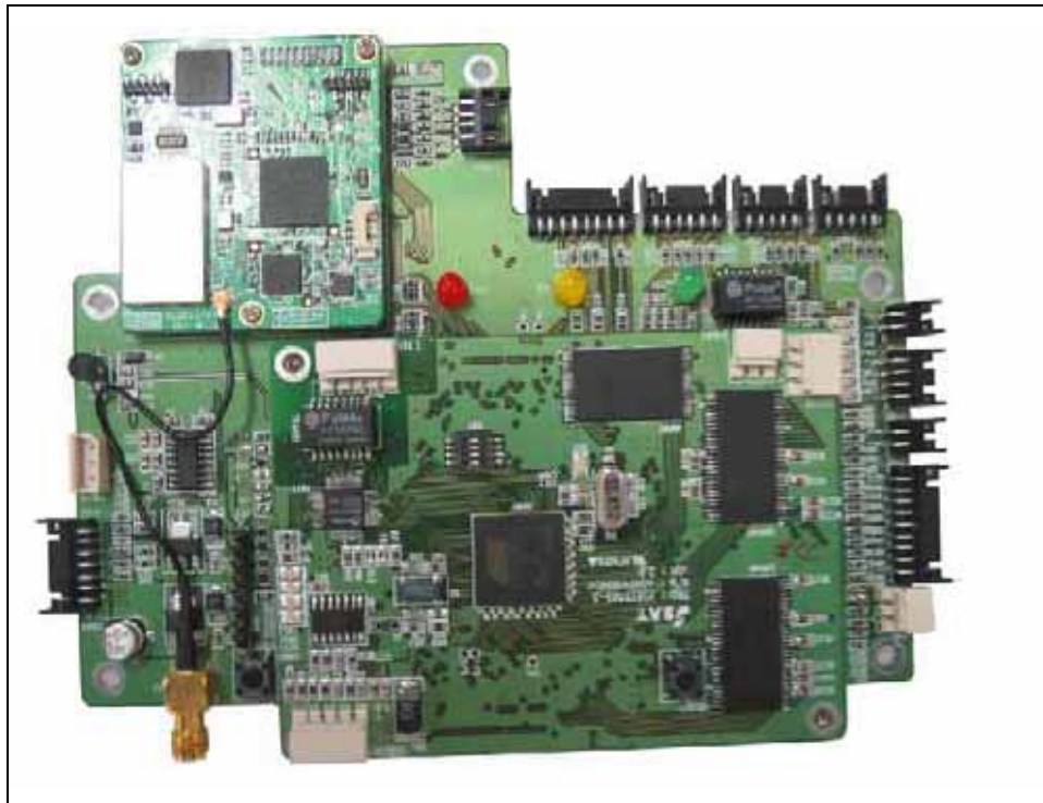
Top view of MCU Board
