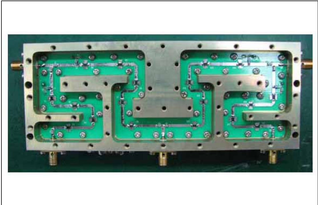
Top view of RF Switch
