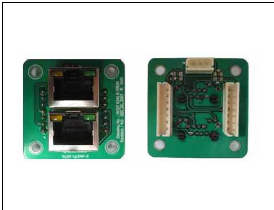
Top & Bottom view of Communication & LED Board
