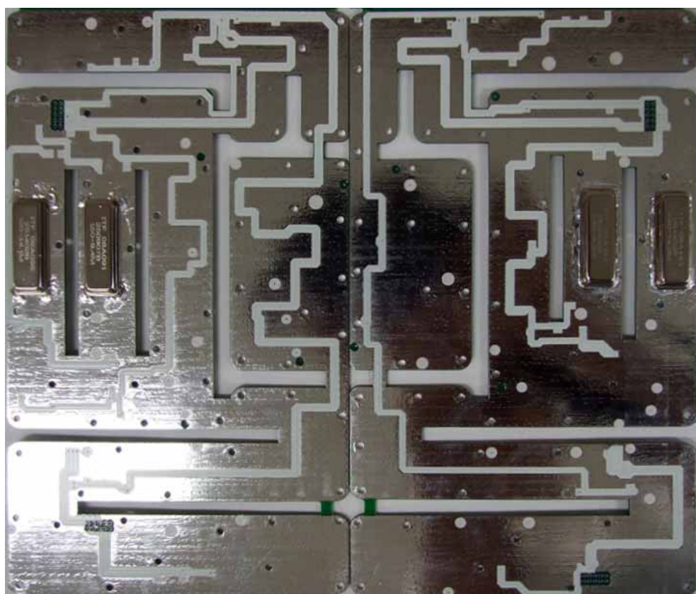
< UDC TOP PCB Bottom View >
