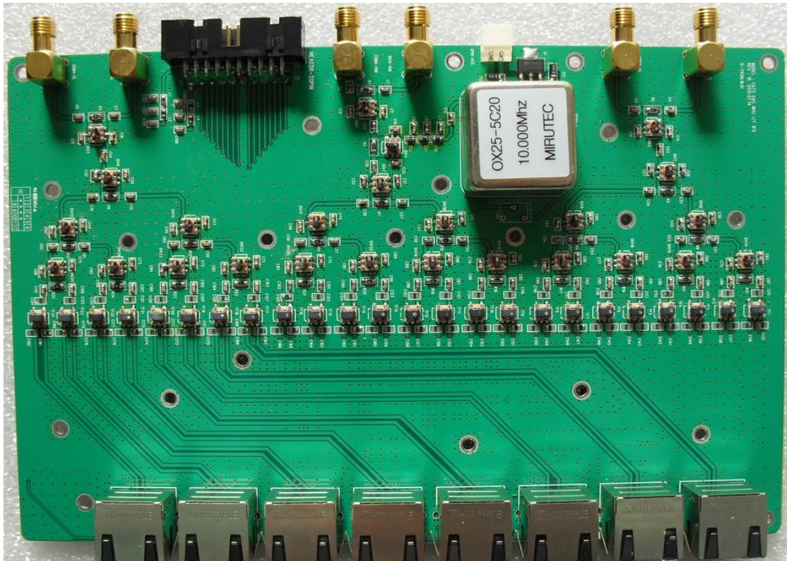
< Interface Board Top view >
