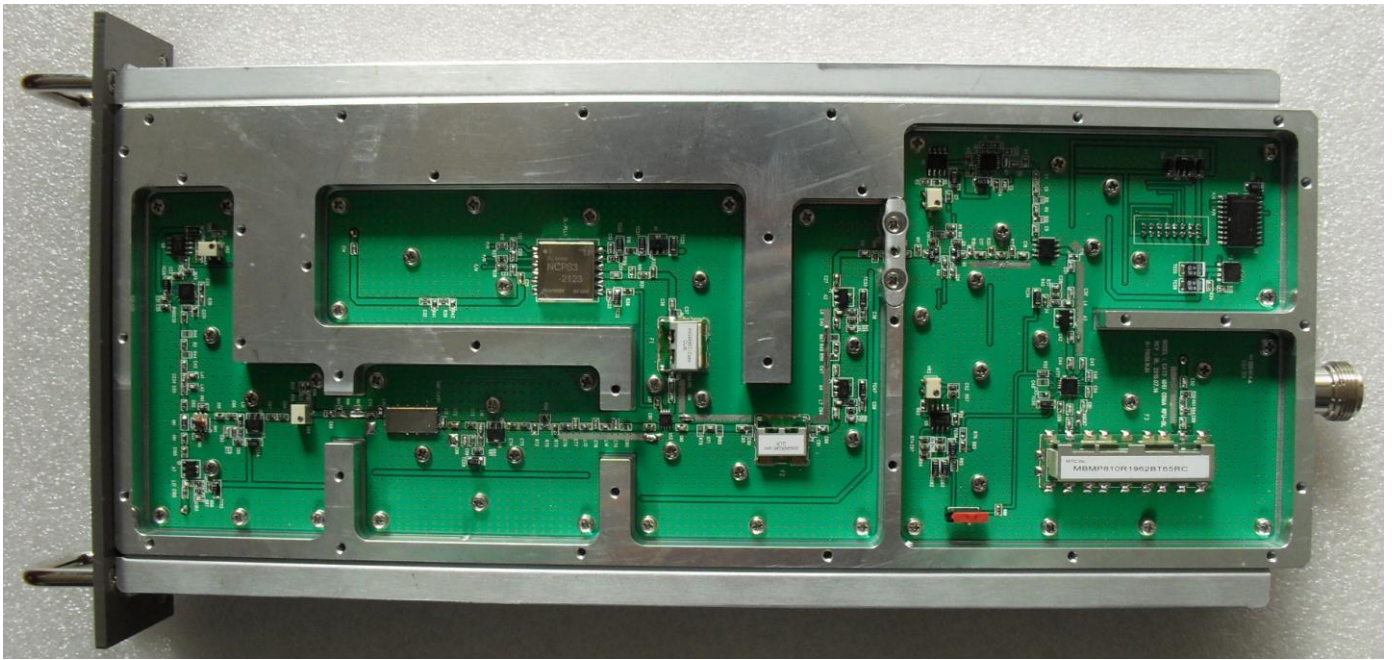
< Bottom View >
