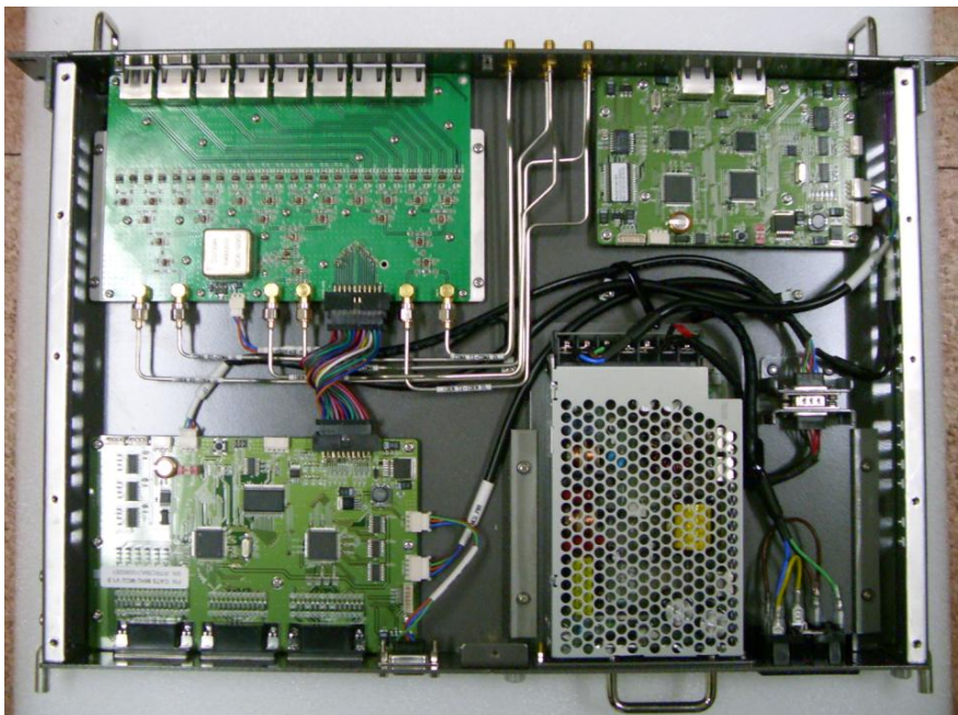
< The Inside of the MHU Main >
