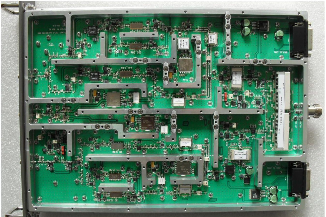
<IDEN RFU Top View>
