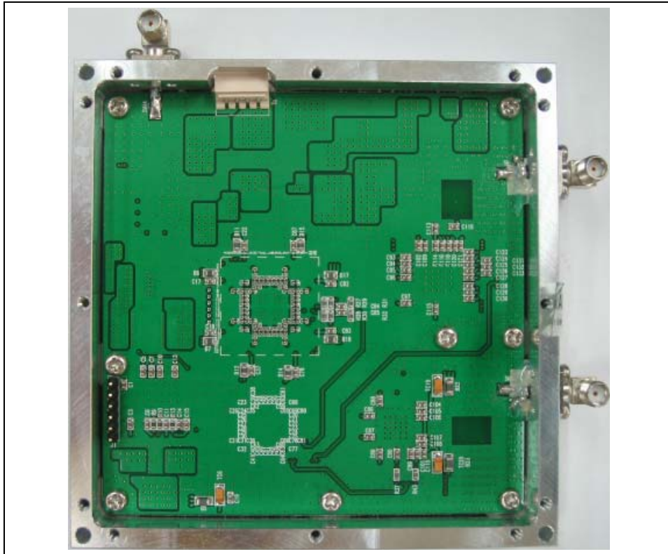
Top view of RF Switch
