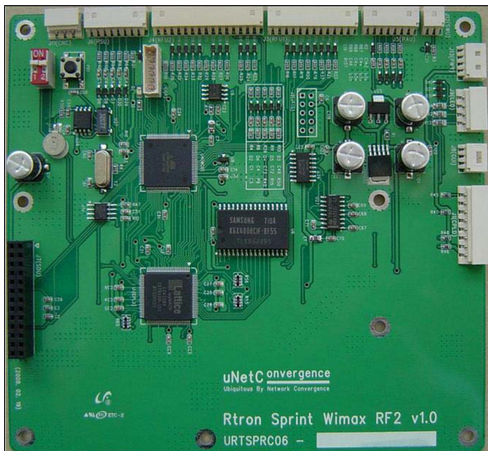
Top view of MCU Board
