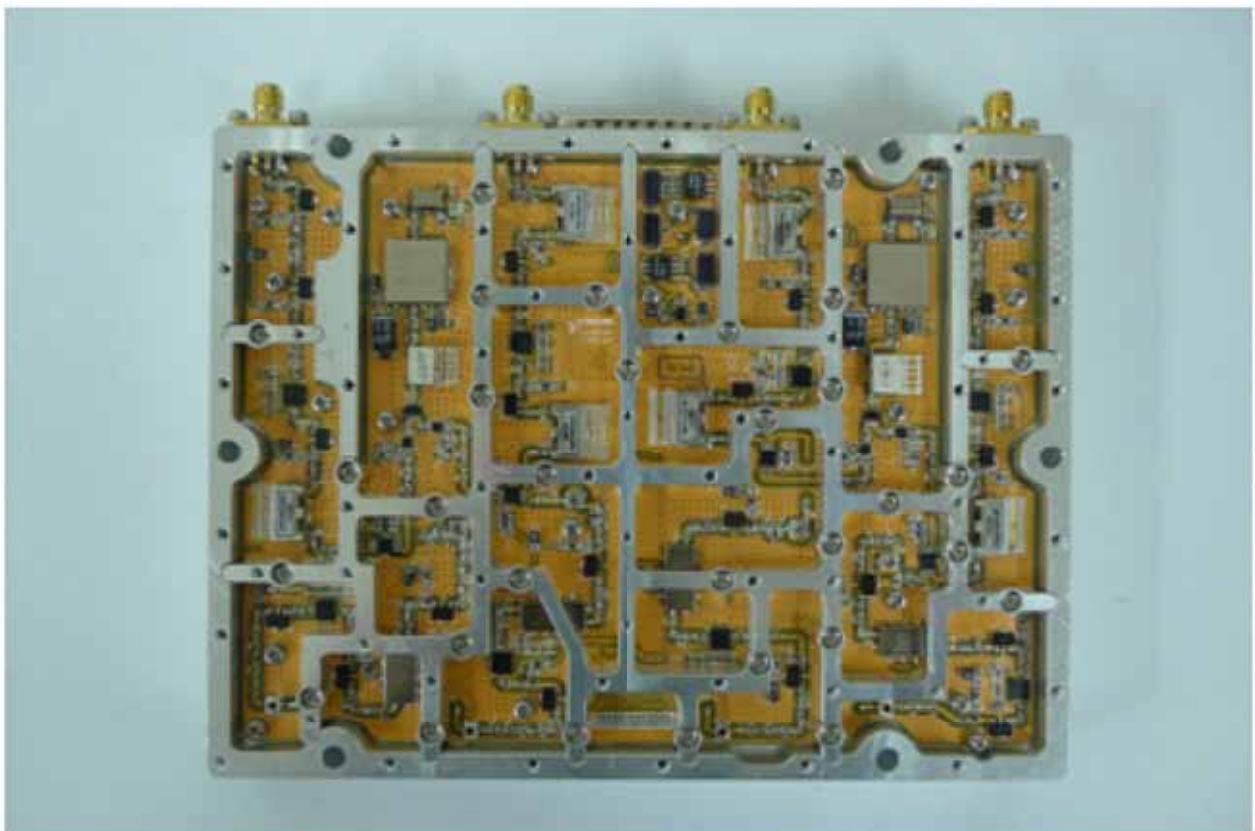
<Top View>
