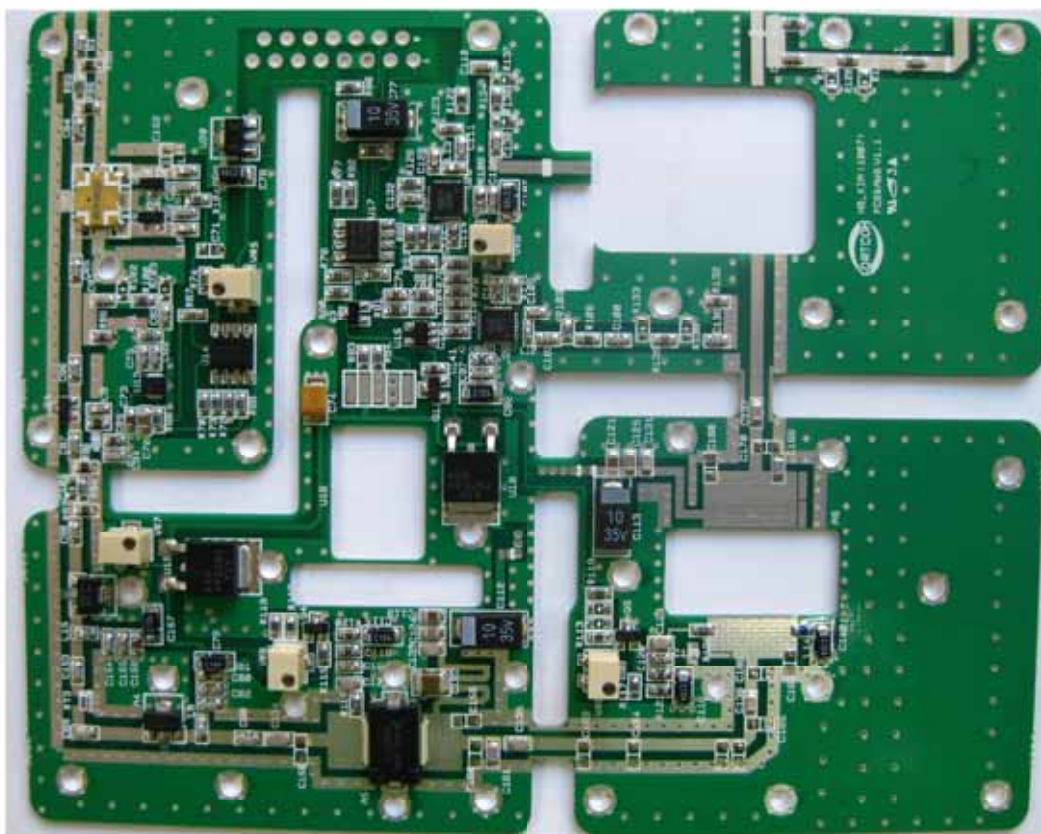
< HPA TOP PCB Top View>
