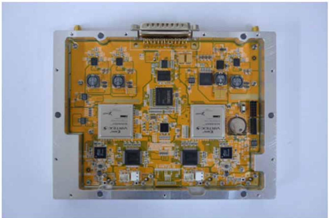
<BOTTOM View>
