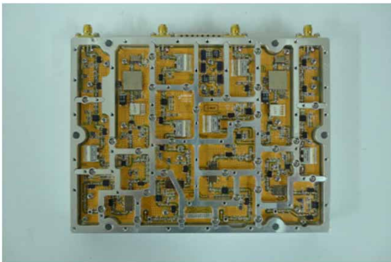
<Top View>
