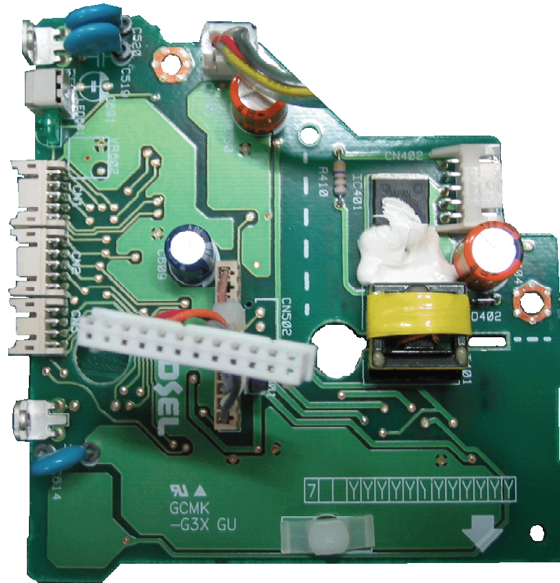
<PSU PCB Top View>
