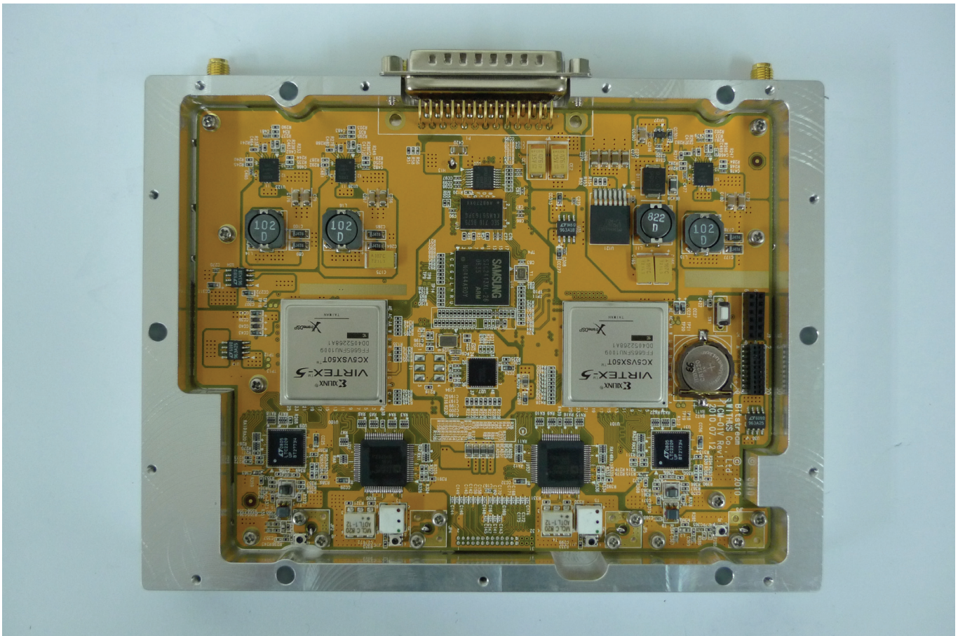
<BOTTOM View>
