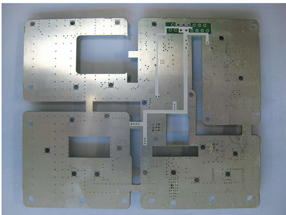
< HPA TOP PCB Bottom View>
