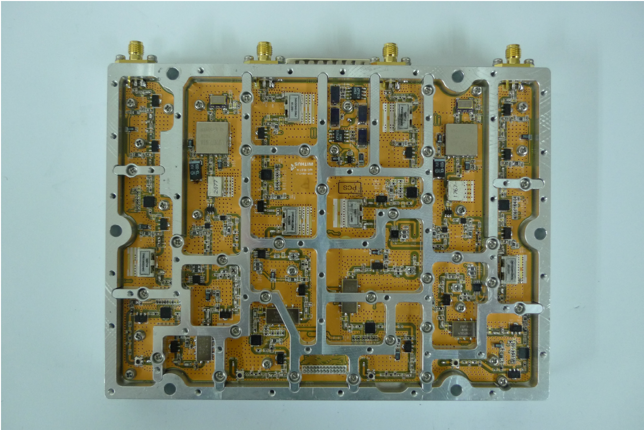
<Top View>
