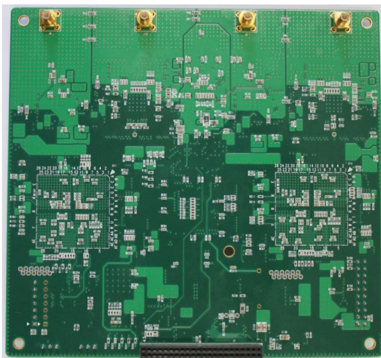
<MCU Bottom View>
