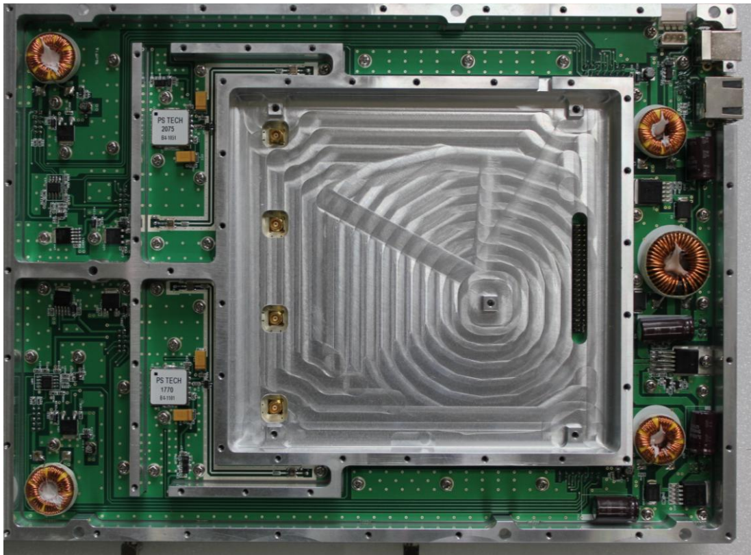
<RFU Bottom view>
