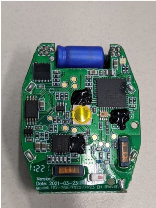
7.4 EUT_ Circuit Board
