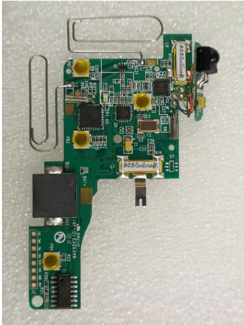
7.4 PCB Component Side View
