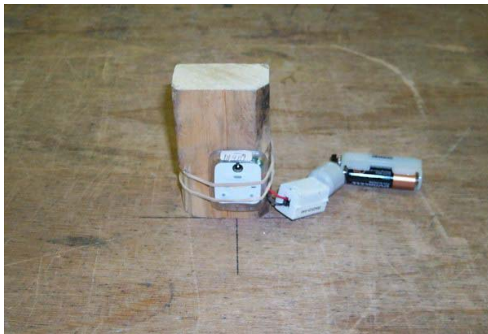
Figure 3.3 Radiated Test Setup, position 3
