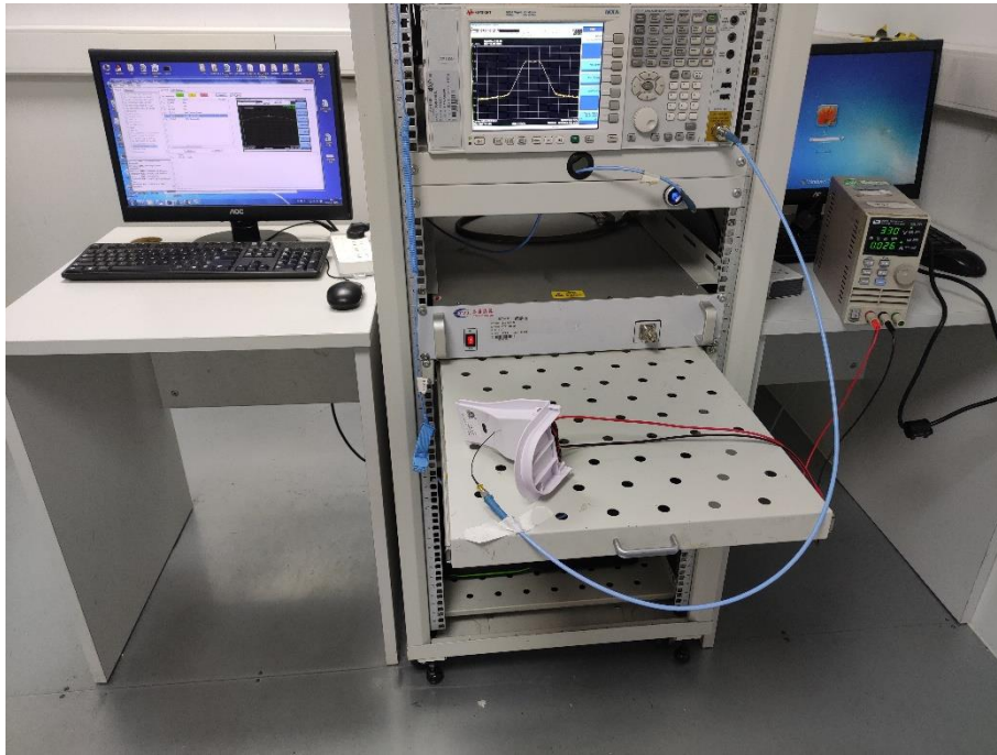
Conducted Test-RFID
