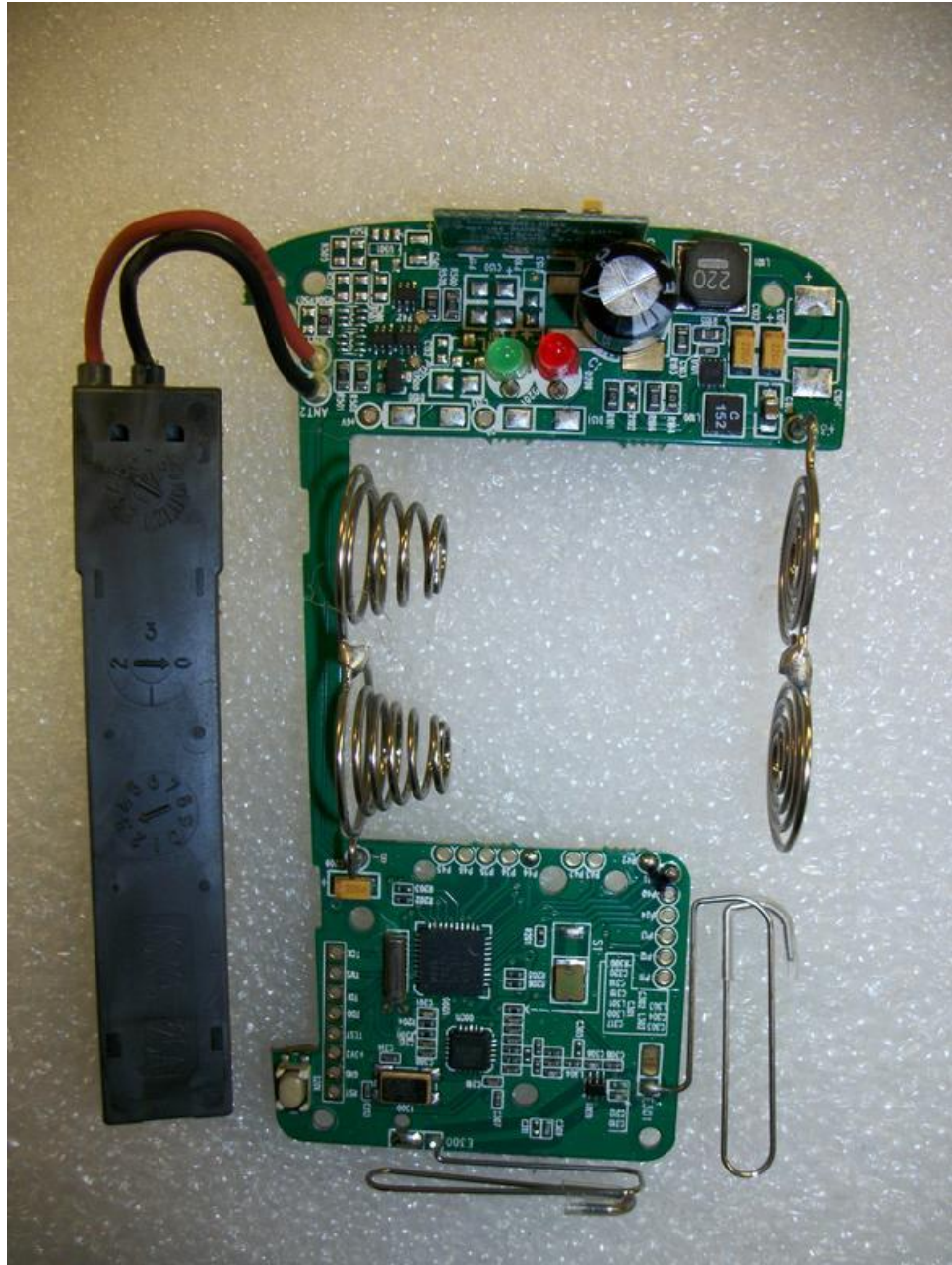
7.4 125KHz Antenna and PCB Component Side View
