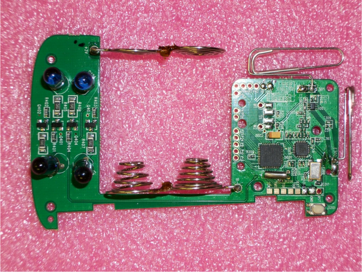
7.4 PCB Component Side View
