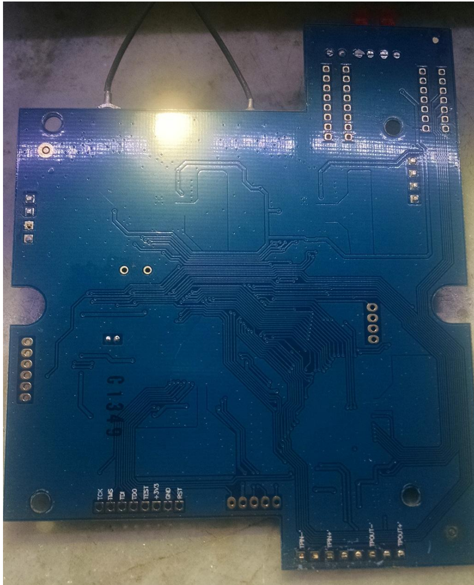
8.7 Main PCB Foil Side View
