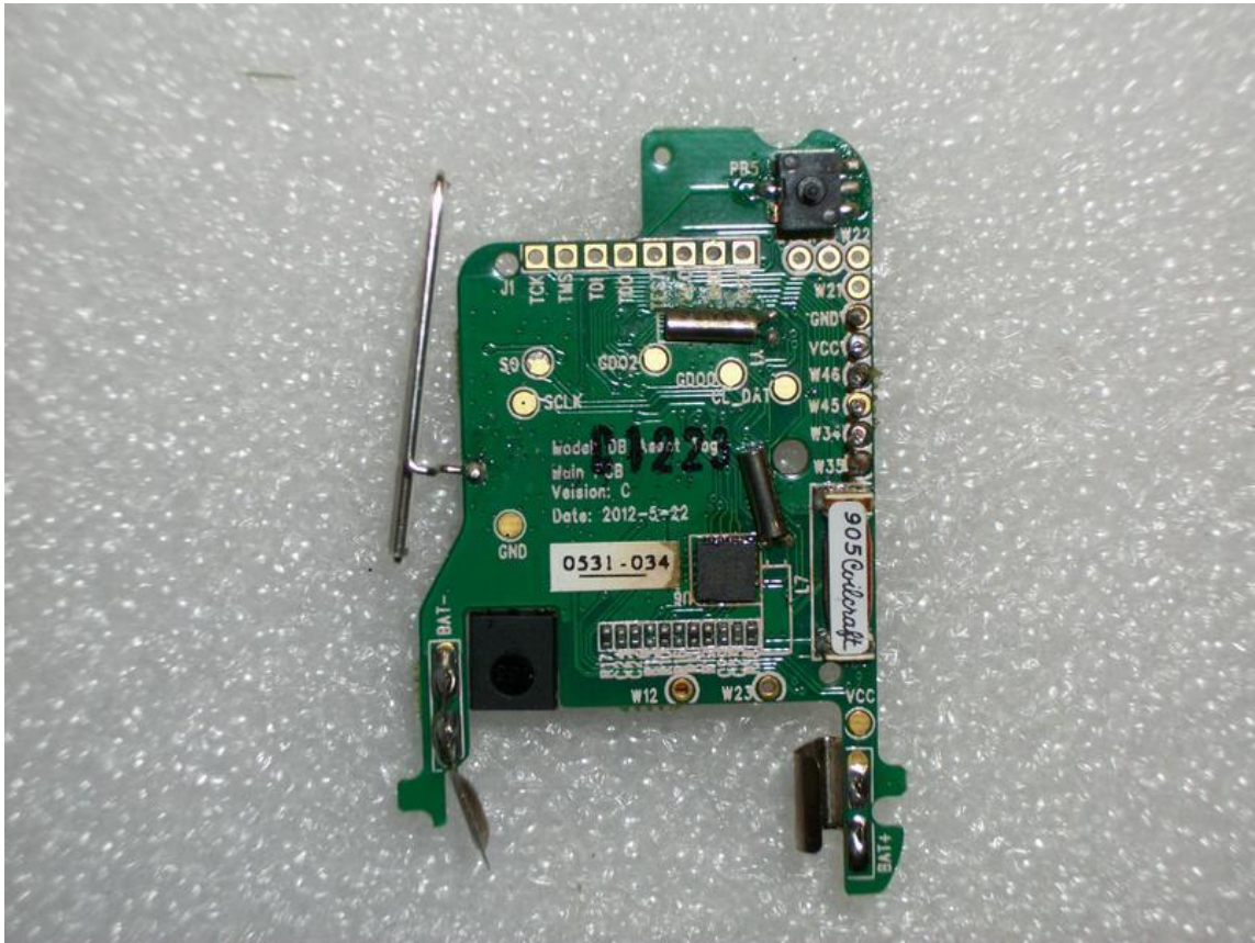
7.5 PCB_900MHz_Component Side 2
