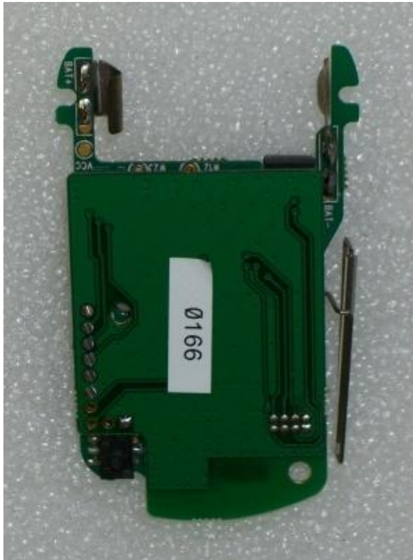
7.7 PCB_2.4G MHz_ Foil View
