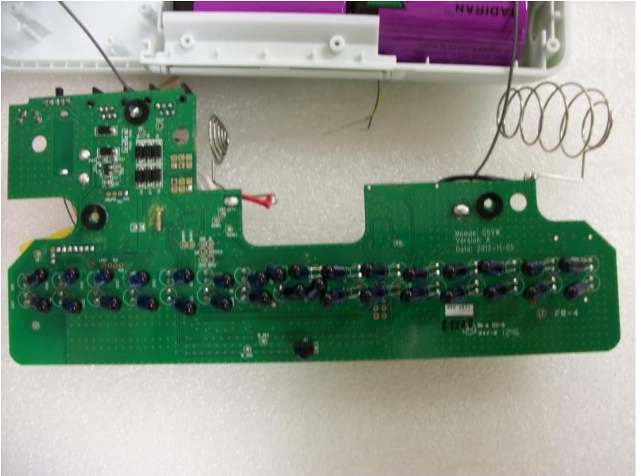
7.5 PCB Foil Side View
