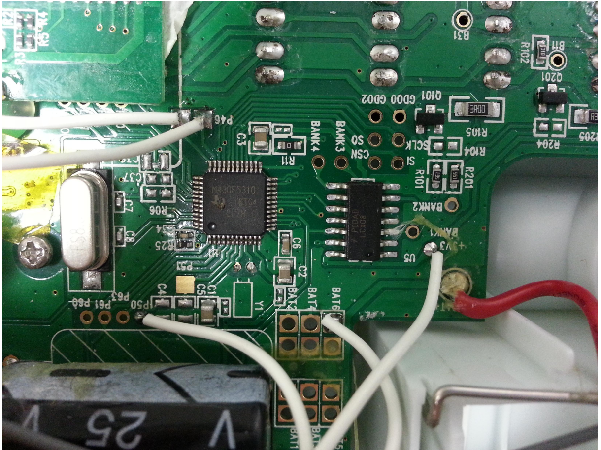
7.11 Close up of the 904-926 MHz transmitter
