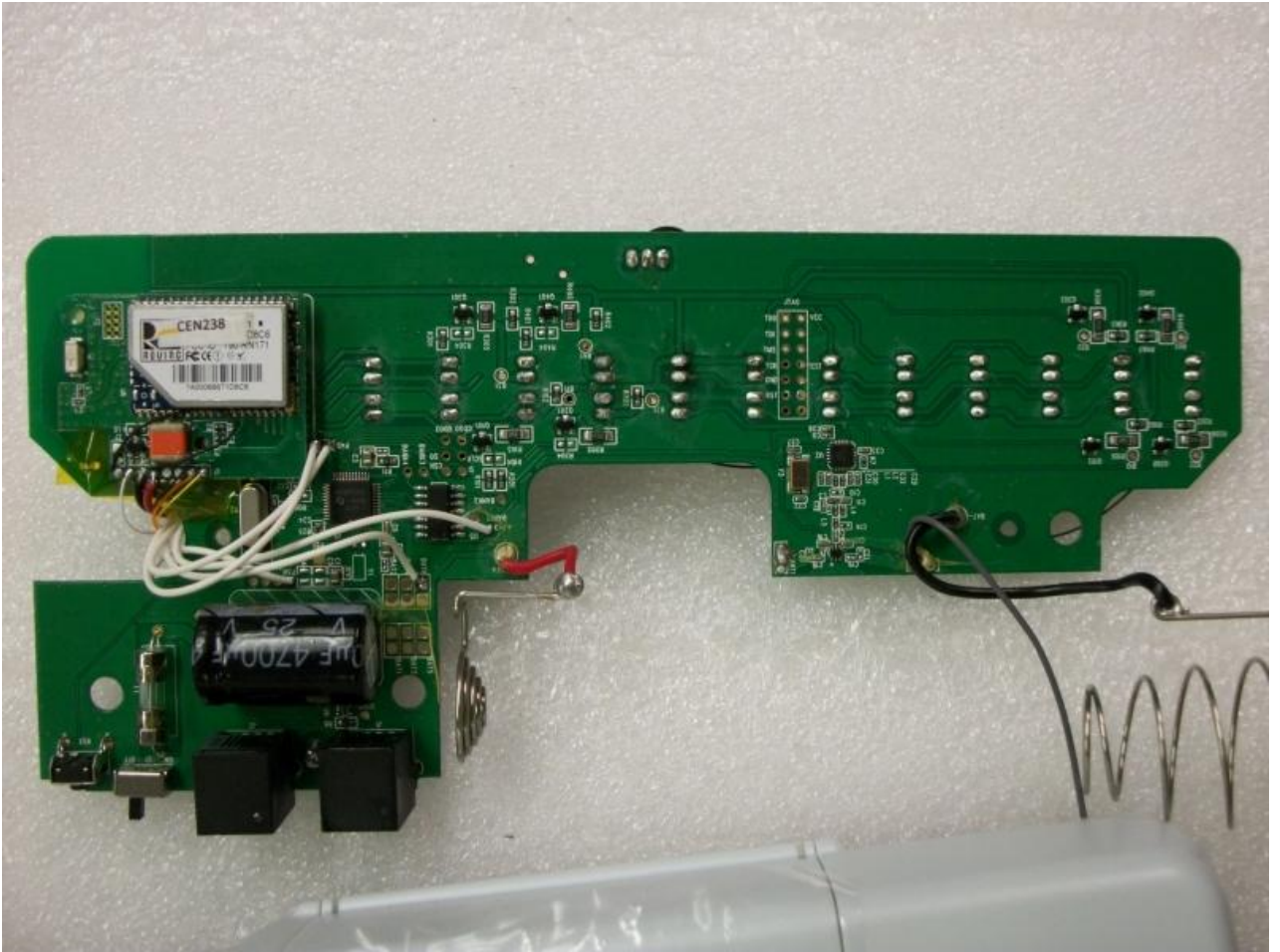
7.4 PCB Component Side View
