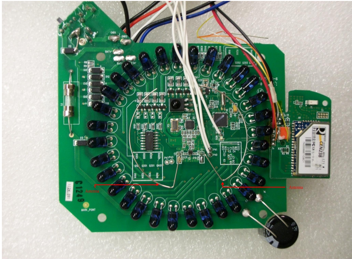
8.5 PCB Component Side View & Antenna Shown up
