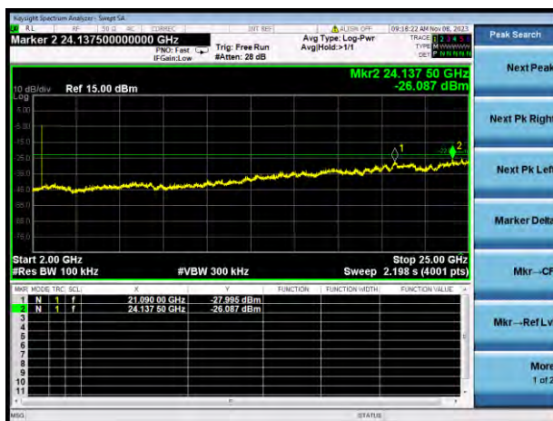
GFSK (BLE 1Mbps) HIGH CHANNEL, SPURIOUS 2 GHz ~ 25 GHz
